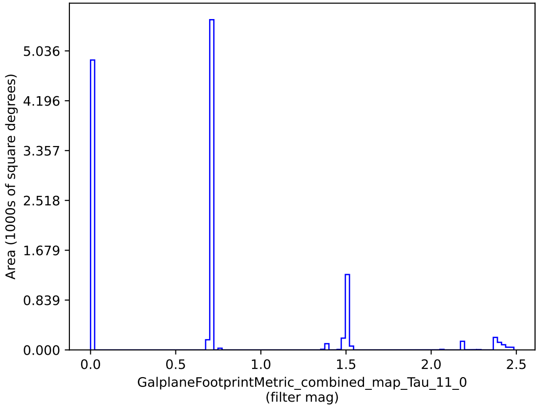
weather_cloudso12v3.4_10yrs : GalplaneFootprintMetric_combined_map_Tau_11_0
