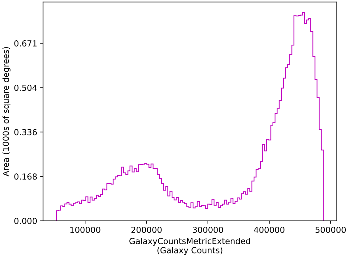
weather_cloudso12v3.4_10yrs z: GalaxyCountsMetricExtended
