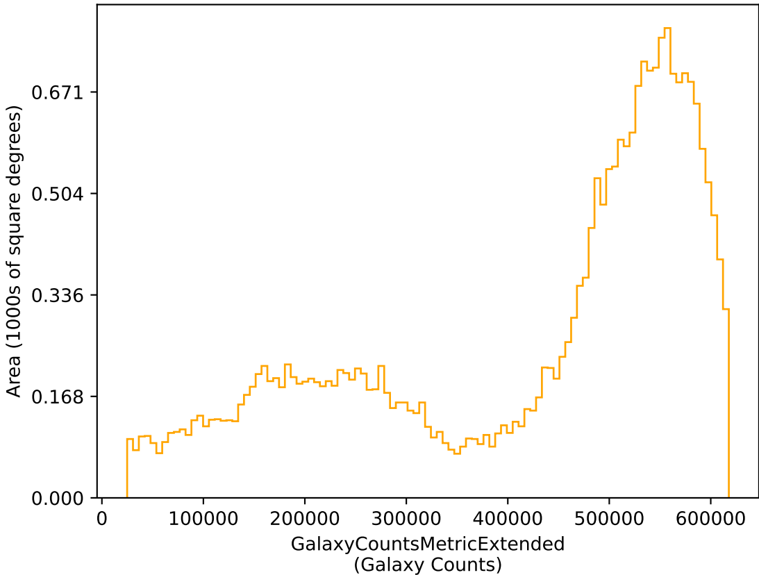
weather_cloudso12v3.4_10yrs r: GalaxyCountsMetricExtended
