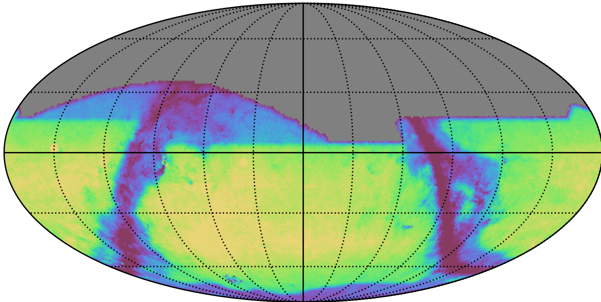
weather_cloudso12v3.4_10yrs i: GalaxyCountsMetricExtended
