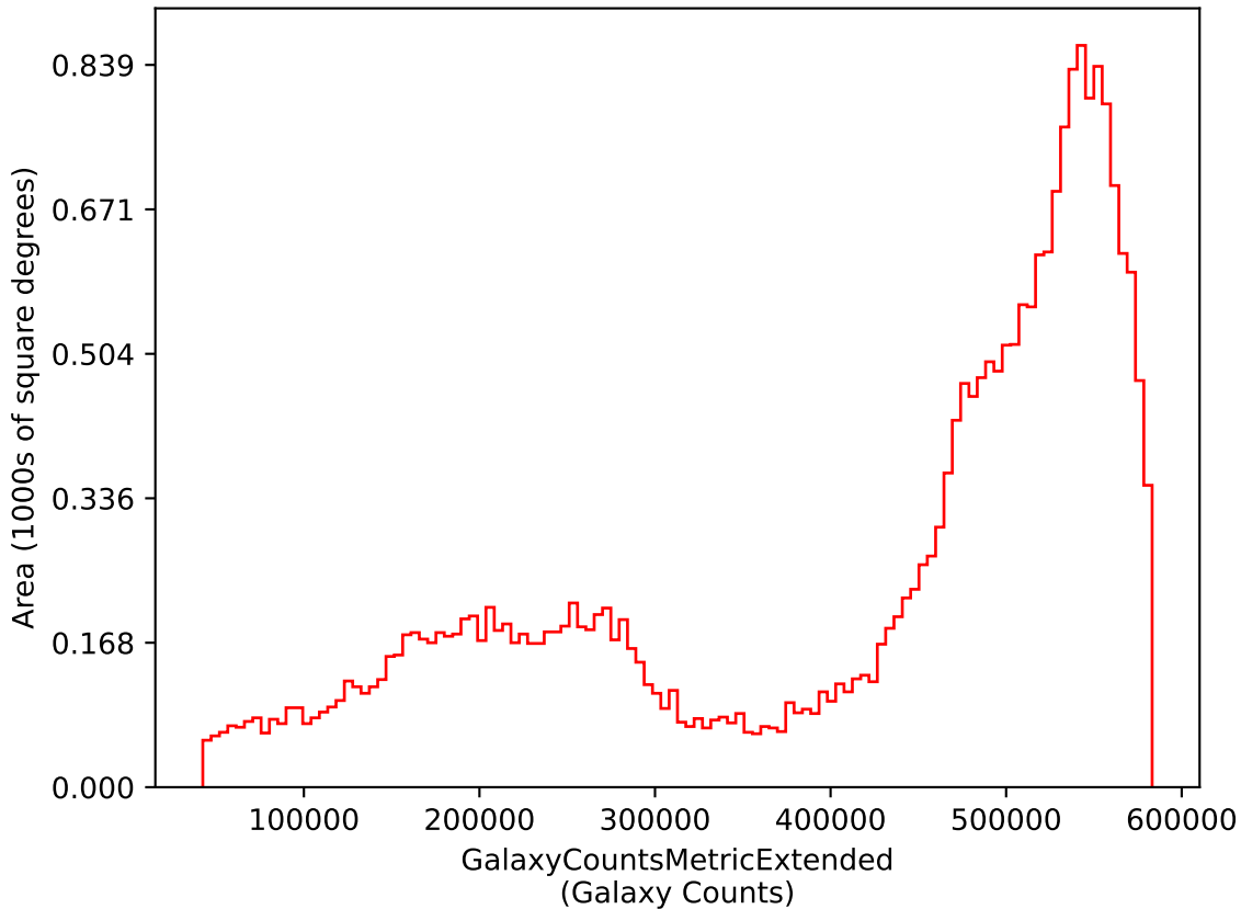
weather_cloudso12v3.4_10yrs i: GalaxyCountsMetricExtended
