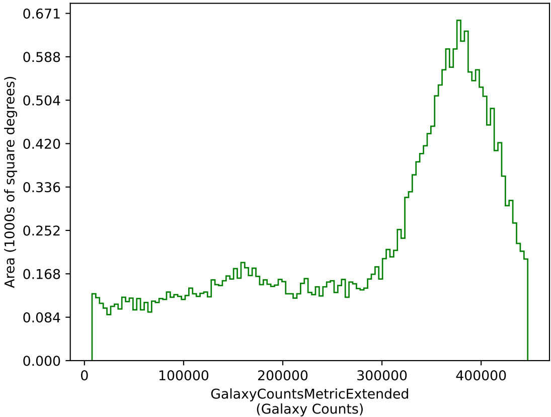
weather_cloudso12v3.4_10yrs g: GalaxyCountsMetricExtended
