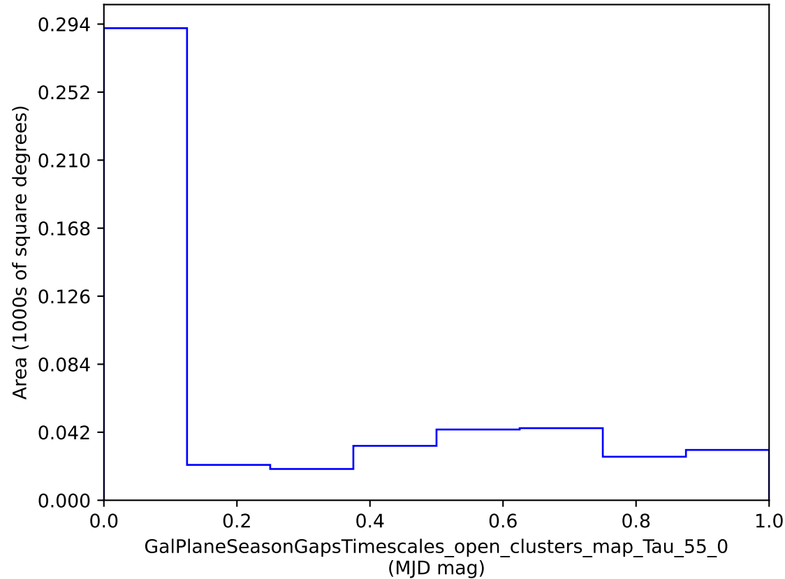
weather_cloudso12v3.4_10yrs : GalPlaneSeasonGapsTimescales_open_clusters_map_Tau_55_0
