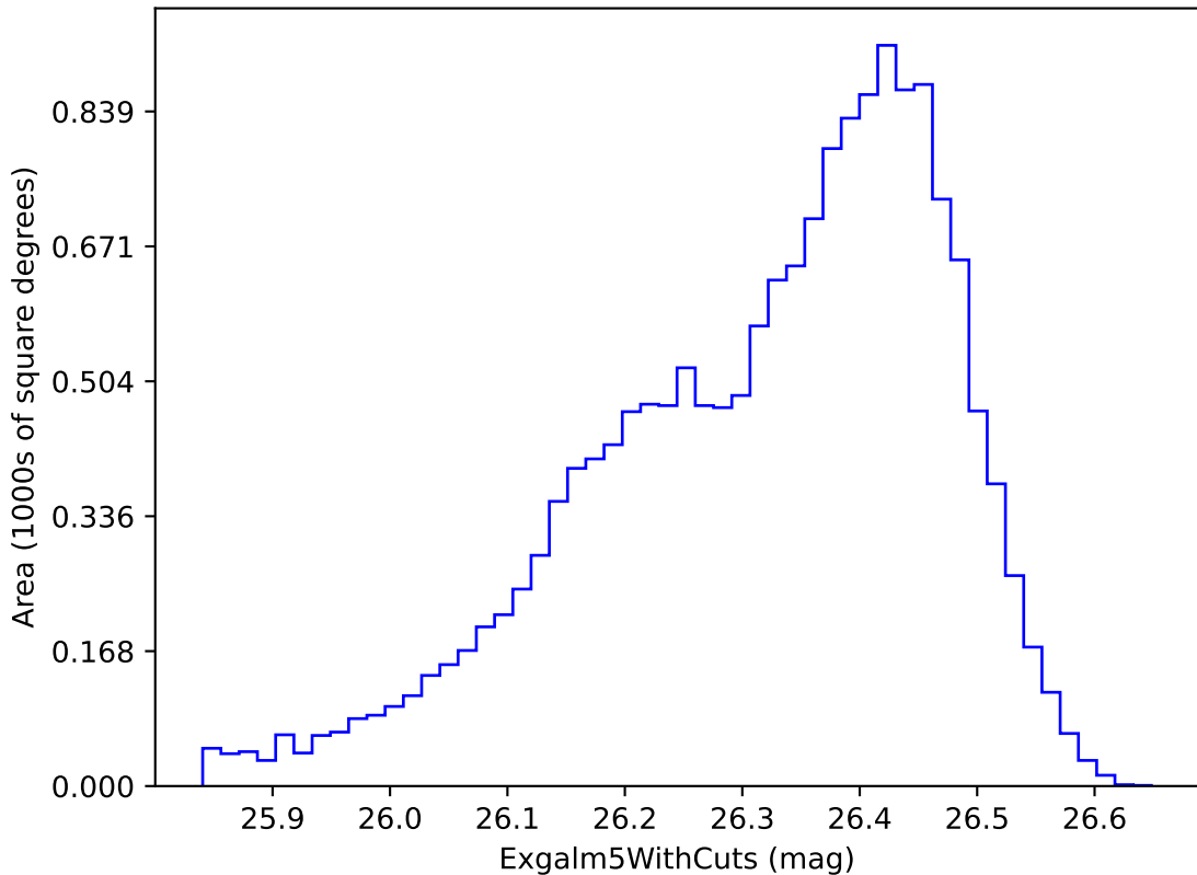
weather_cloudso12v3.4_10yrs i band non-DD year 9: ExgalM5WithCuts
