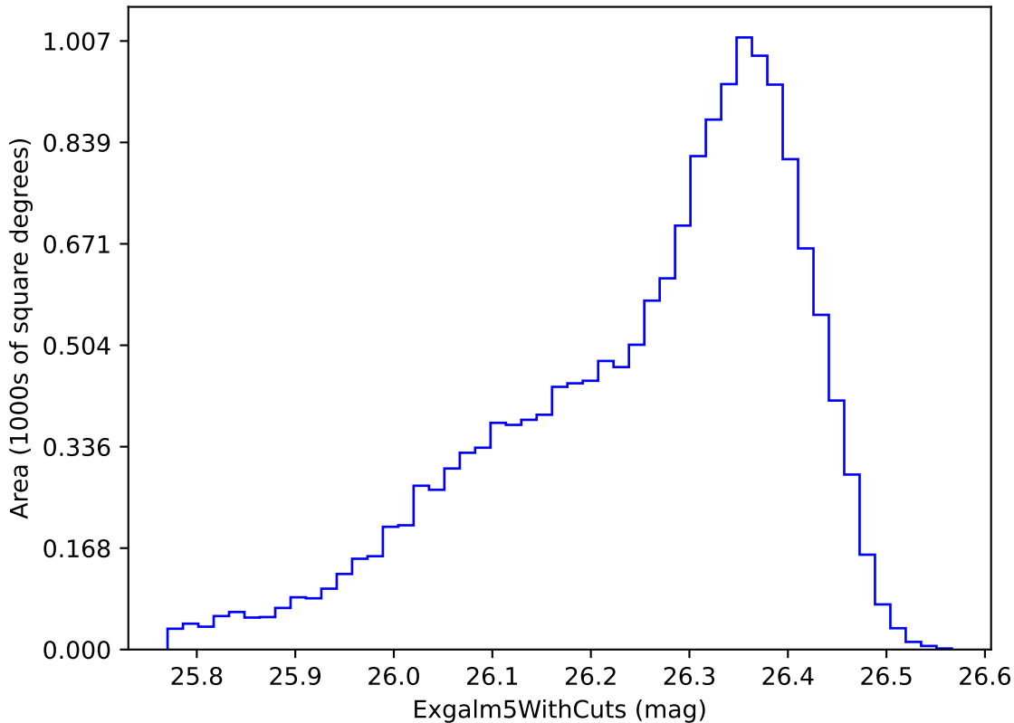
weather_cloudso12v3.4_10yrs i band non-DD year 8: ExgalM5WithCuts
