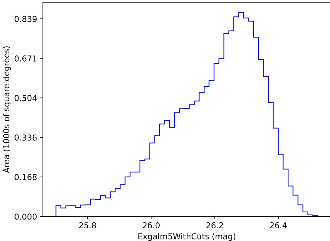
weather_cloudso12v3.4_10yrs i band non-DD year 7: ExgalM5WithCuts
