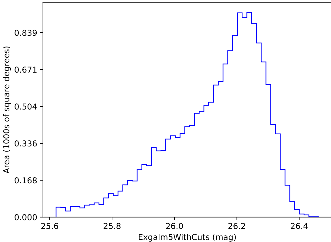
weather_cloudso12v3.4_10yrs i band non-DD year 6: ExgalM5WithCuts
