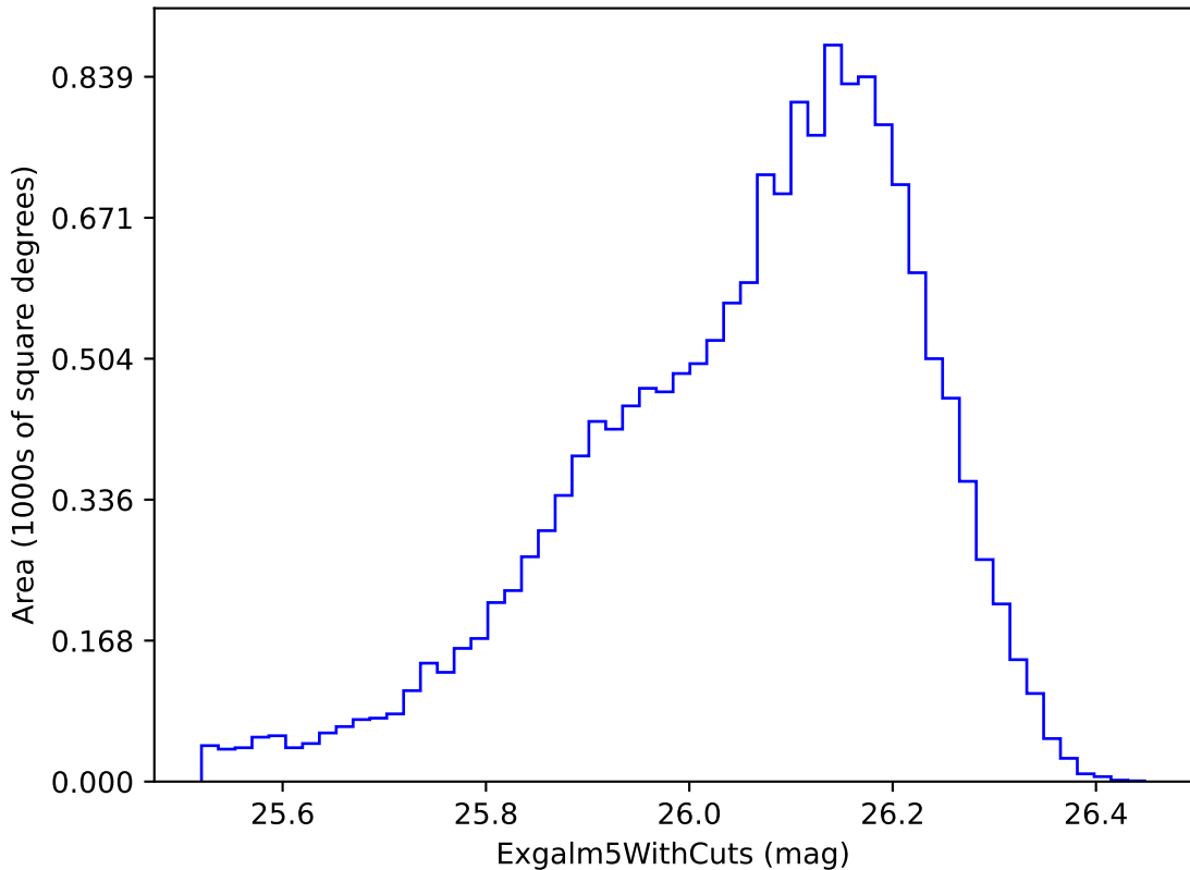
weather_cloudso12v3.4_10yrs i band non-DD year 5: ExgalM5WithCuts
