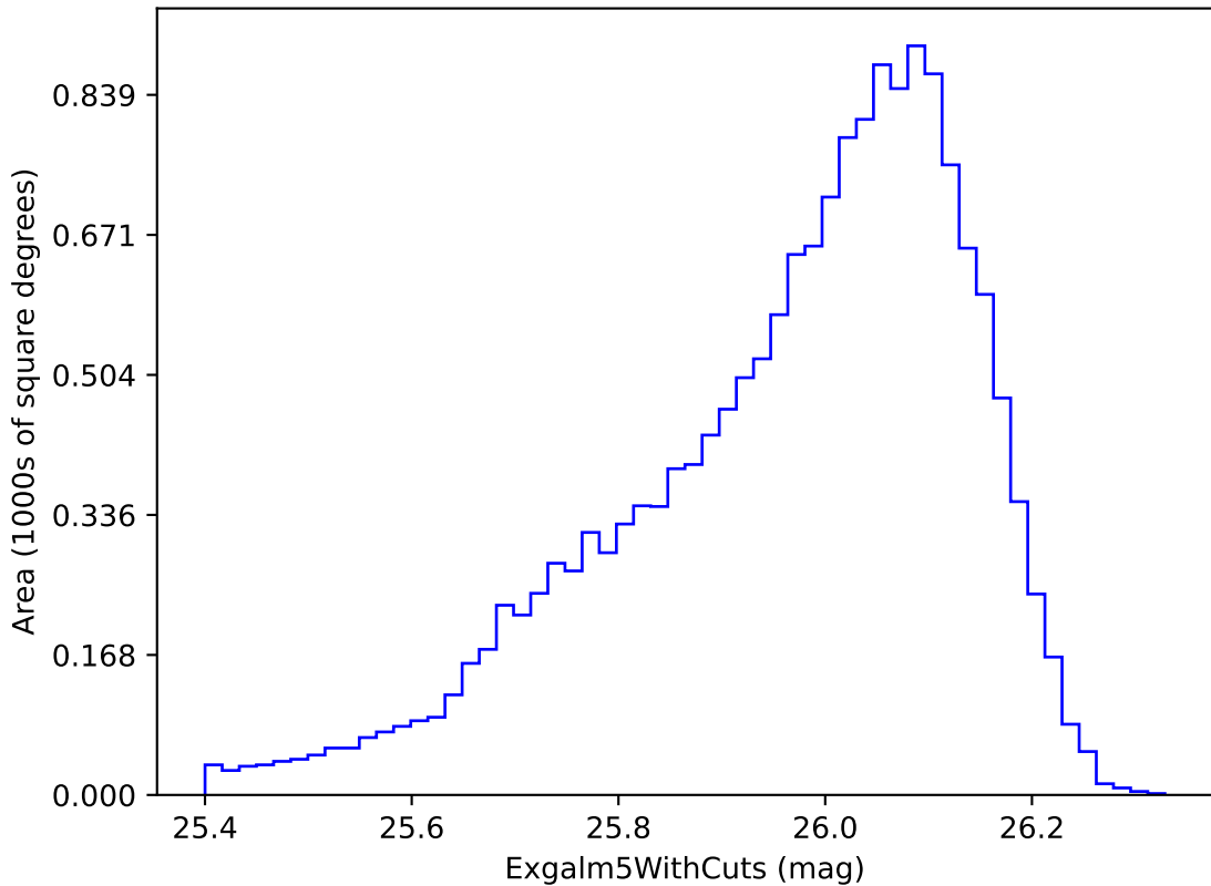
weather_cloudso12v3.4_10yrs i band non-DD year 4: ExgalM5WithCuts
