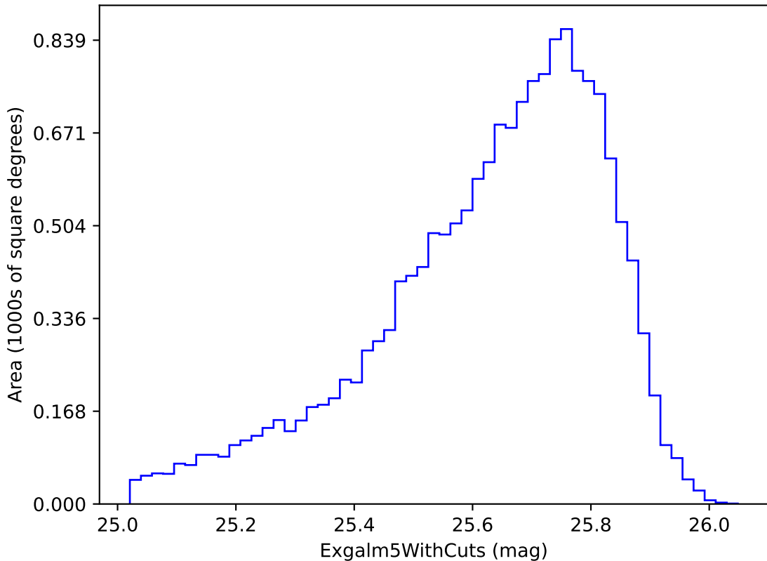
weather_cloudso12v3.4_10yrs i band non-DD year 2: ExgalM5WithCuts
