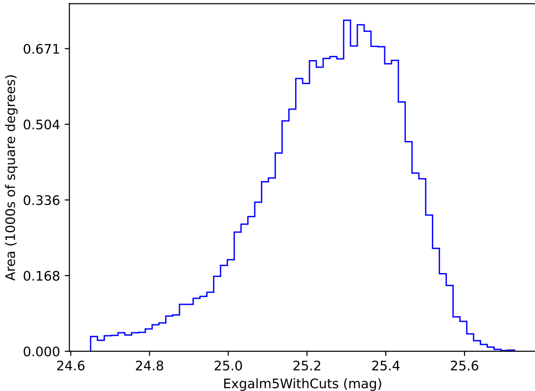
weather_cloudso12v3.4_10yrs i band non-DD year 1: ExgalM5WithCuts
