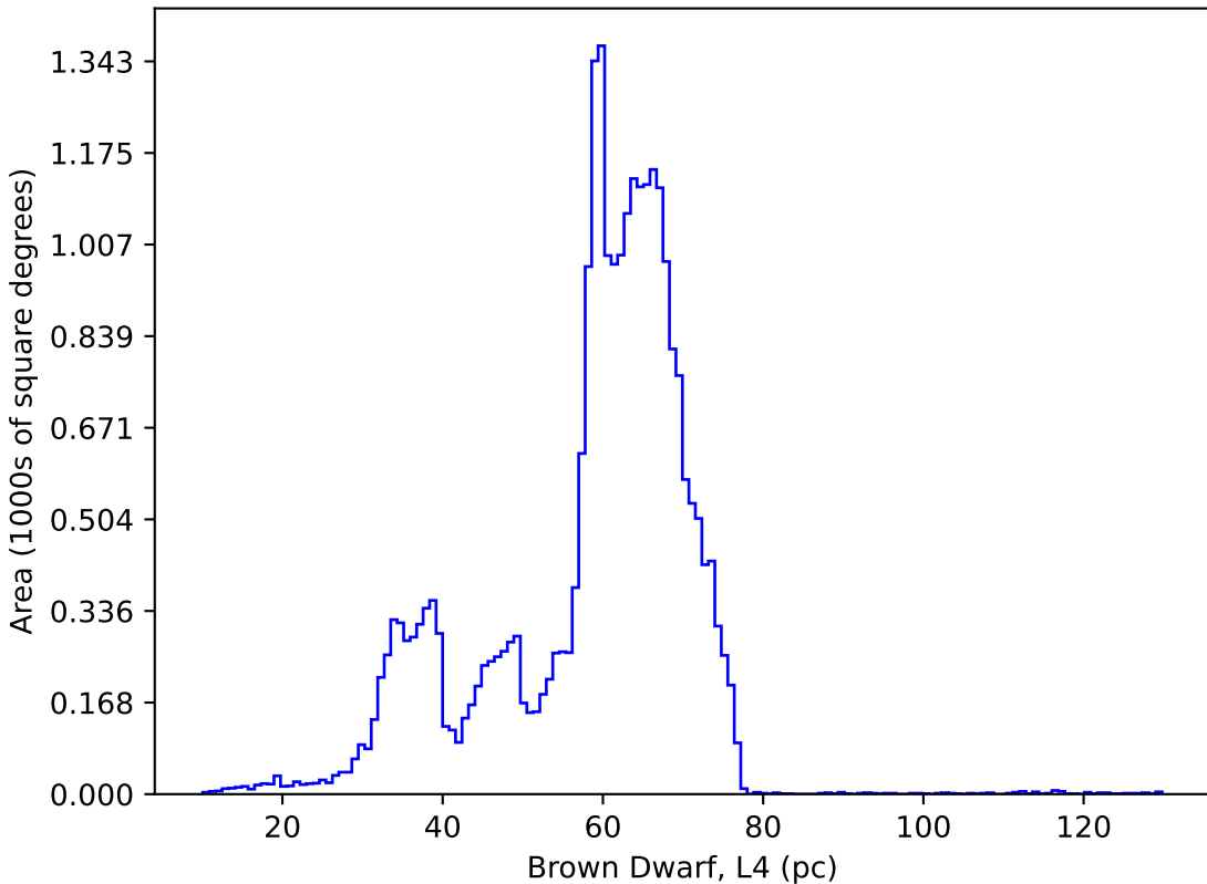
weather_cloudso12v3.4_10yrs : Brown Dwarf, L4
