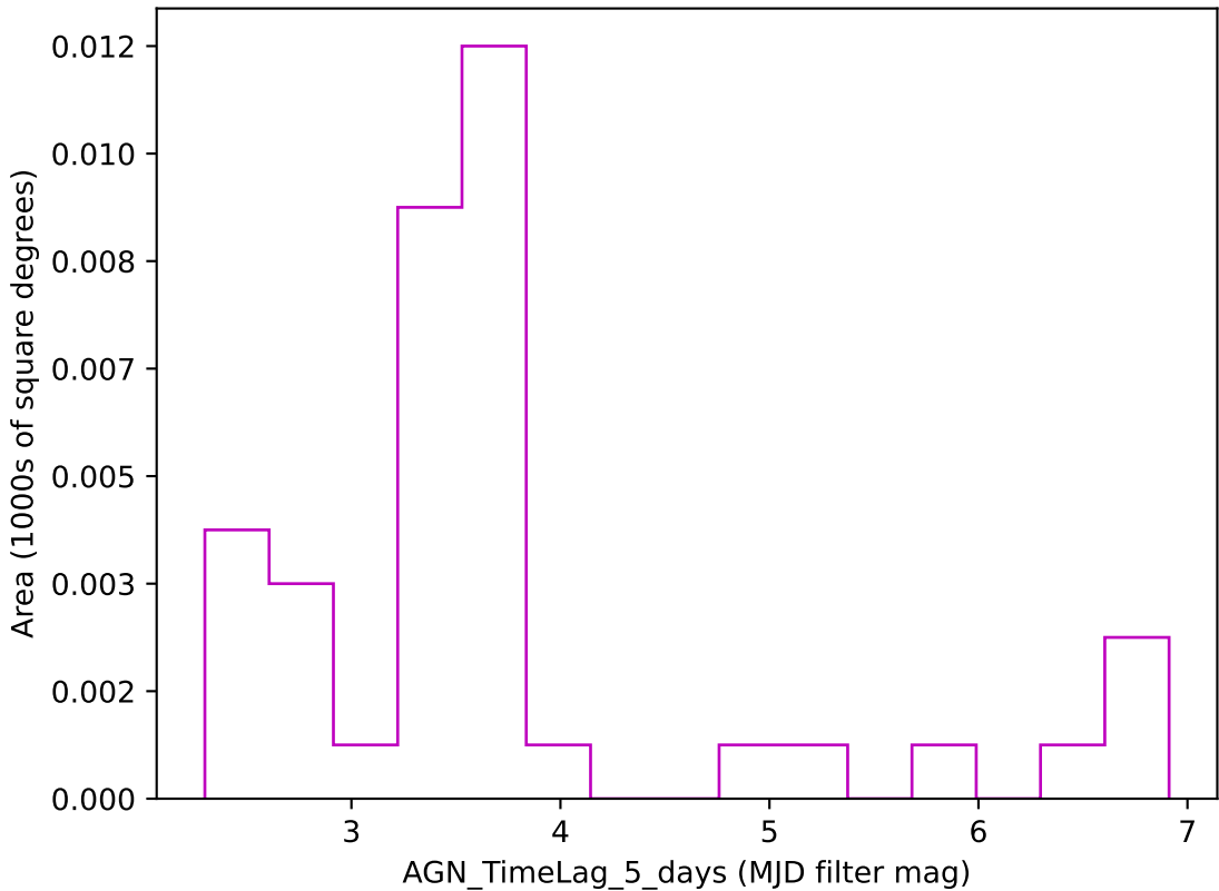
weather_cloudso12v3.4_10yrs z band: AGN_TimeLag_5_days
