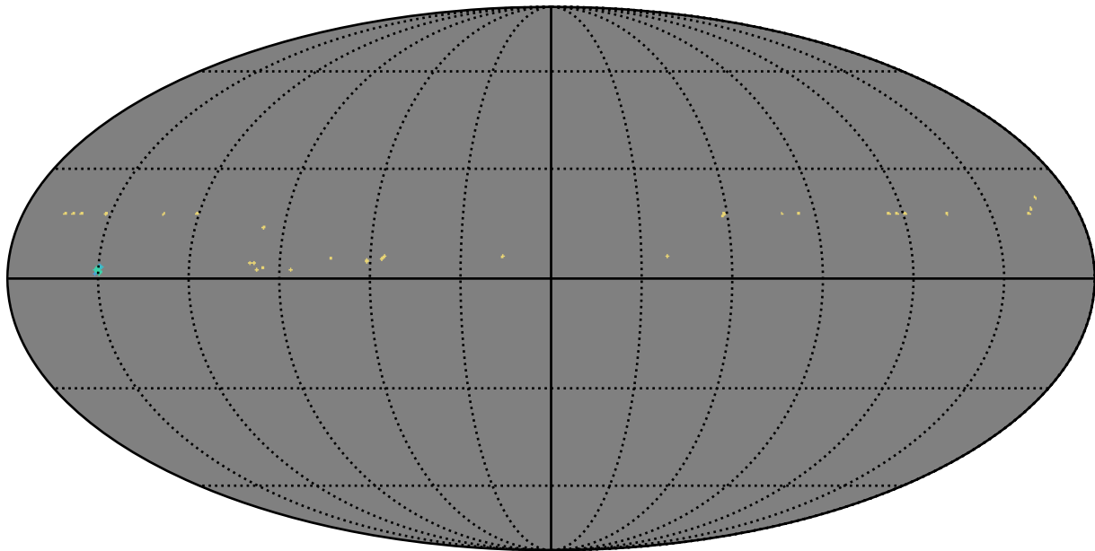
weather_cloudso12v3.4_10yrs y band: AGN_TimeLag_5_days
