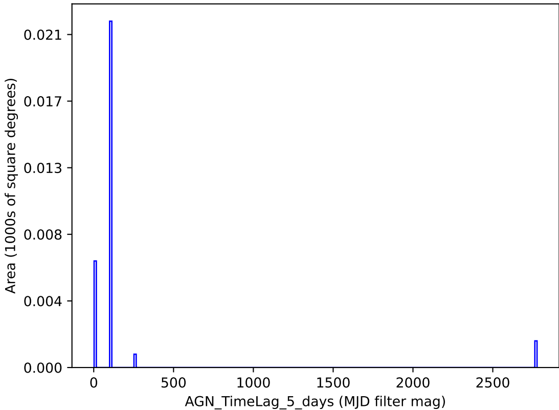
weather_cloudso12v3.4_10yrs y band: AGN_TimeLag_5_days
