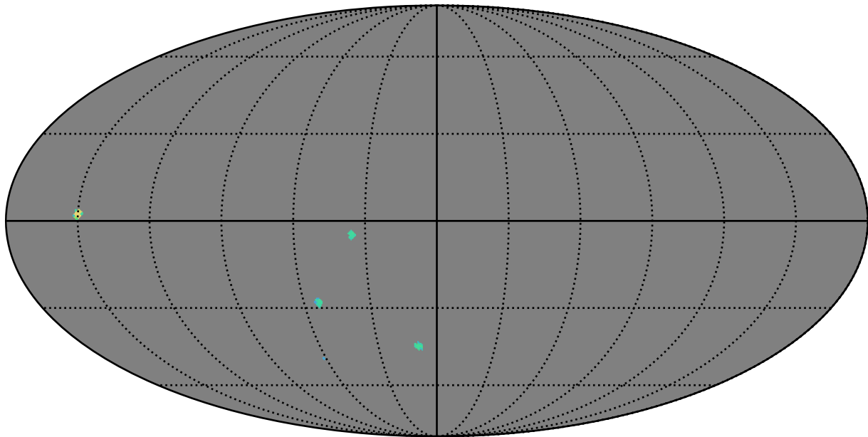
weather_cloudso12v3.4_10yrs r band: AGN_TimeLag_5_days
