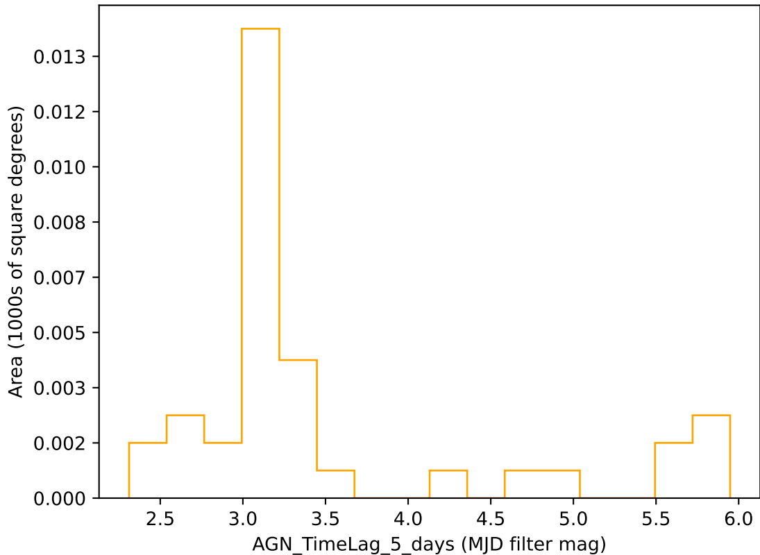
weather_cloudso12v3.4_10yrs r band: AGN_TimeLag_5_days
