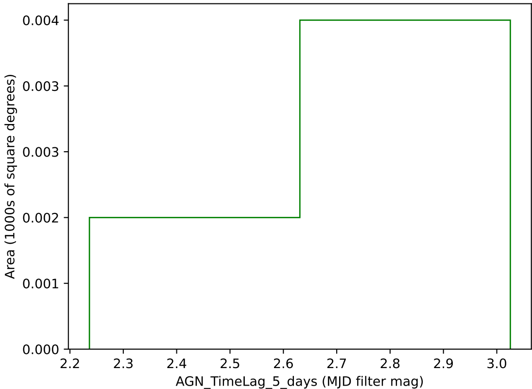
weather_cloudso12v3.4_10yrs g band: AGN_TimeLag_5_days
