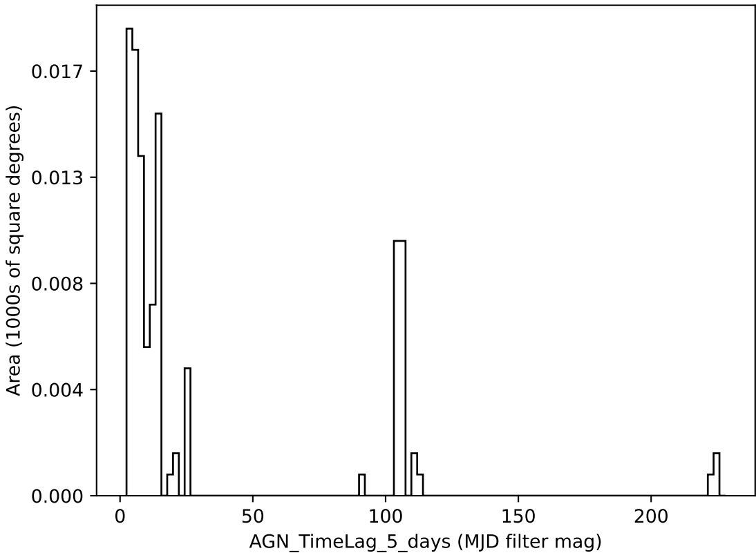
weather_cloudso12v3.4_10yrs all bands: AGN_TimeLag_5_days
