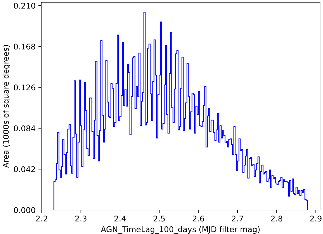
weather_cloudso12v3.4_10yrs y band: AGN_TimeLag_100_days
