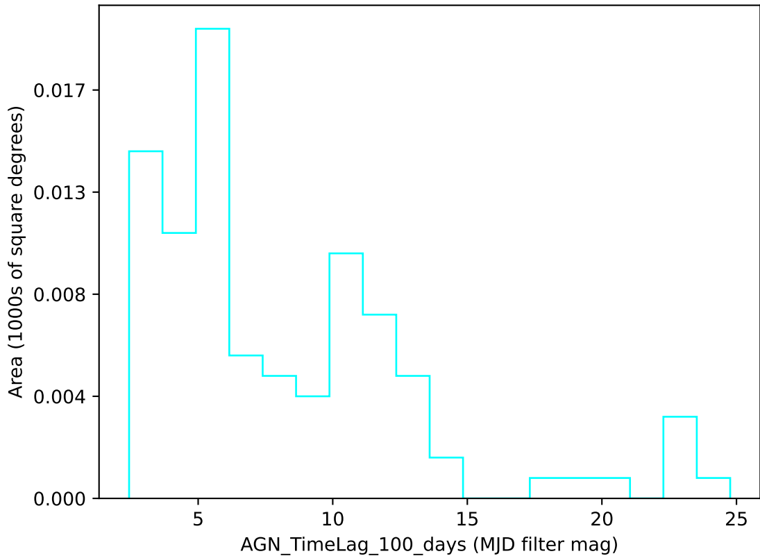
weather_cloudso12v3.4_10yrs u band: AGN_TimeLag_100_days
