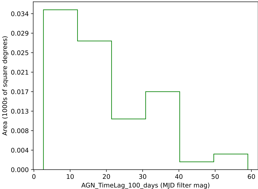
weather_cloudso12v3.4_10yrs g band: AGN_TimeLag_100_days
