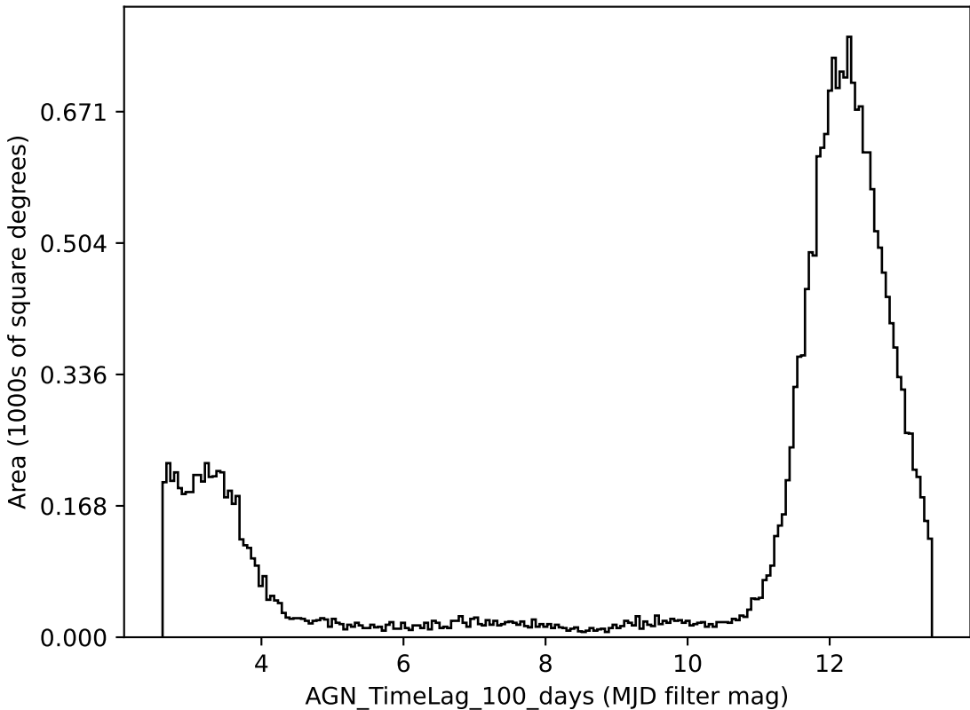
weather_cloudso12v3.4_10yrs all bands: AGN_TimeLag_100_days
