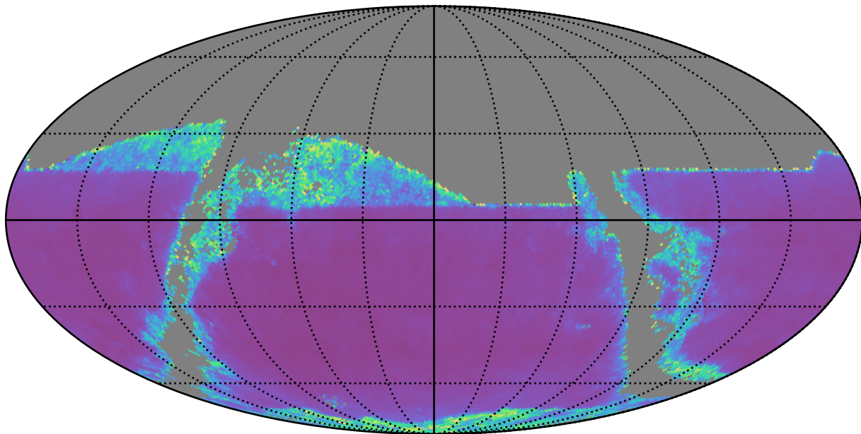
weather_cloudso12v3.4_10yrs z band: AGN SF_uncert
