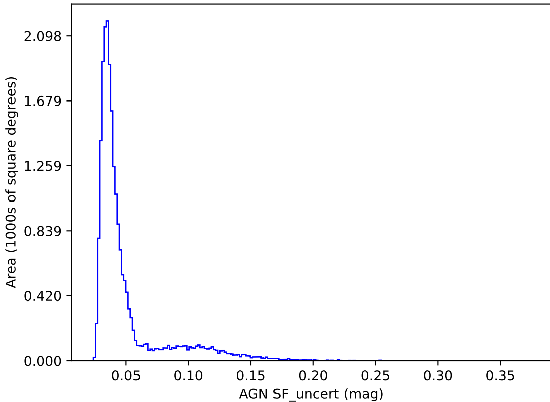
weather_cloudso12v3.4_10yrs y band: AGN SF_uncert
