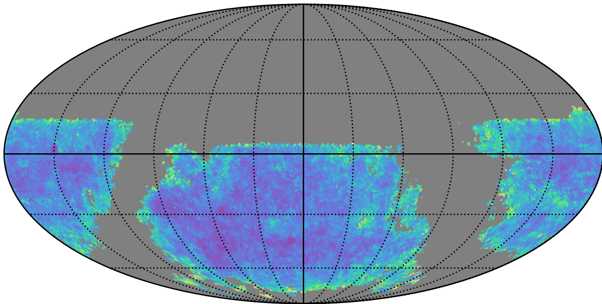
weather_cloudso12v3.4_10yrs u band: AGN SF_uncert
