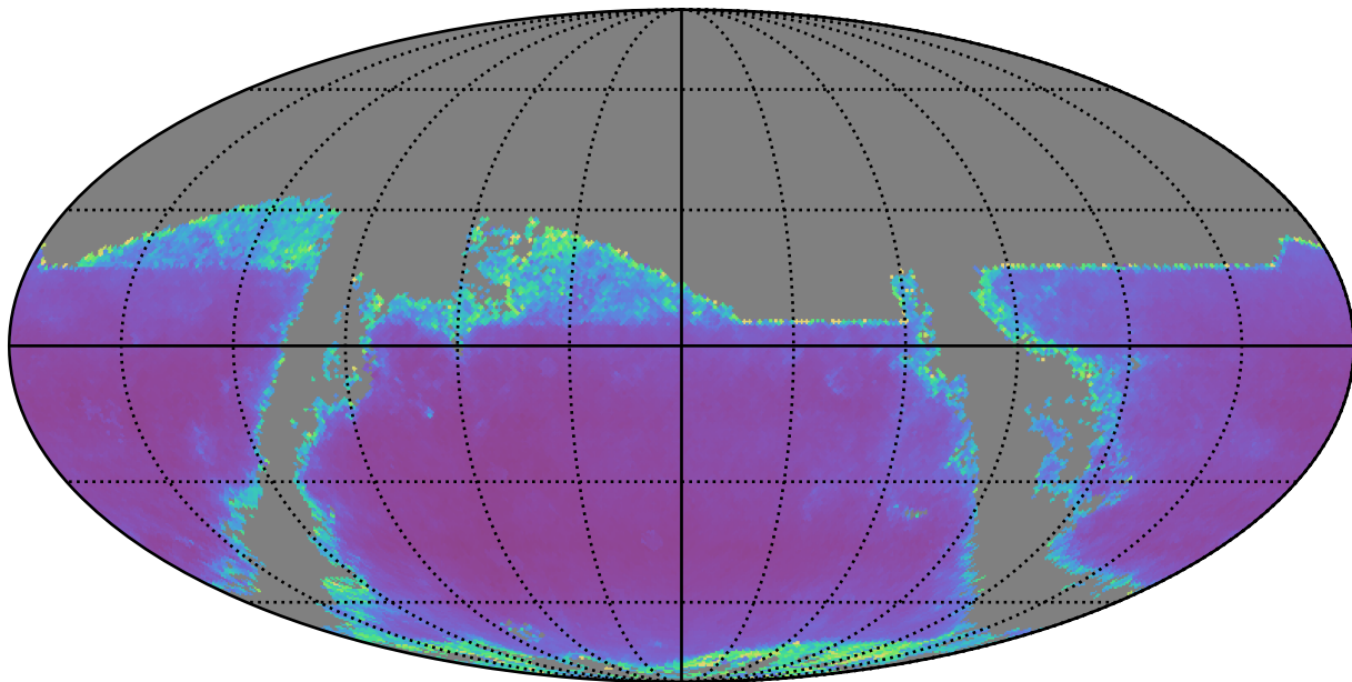
weather_cloudso12v3.4_10yrs r band: AGN SF_uncert
