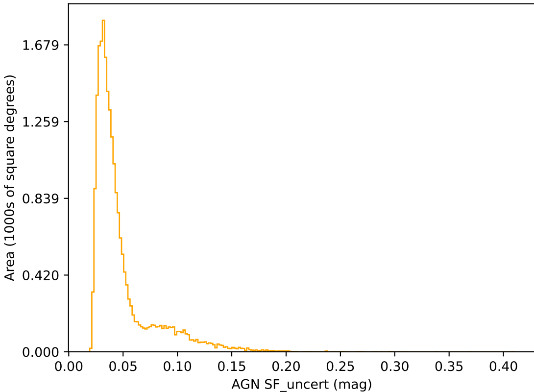
weather_cloudso12v3.4_10yrs r band: AGN SF_uncert
