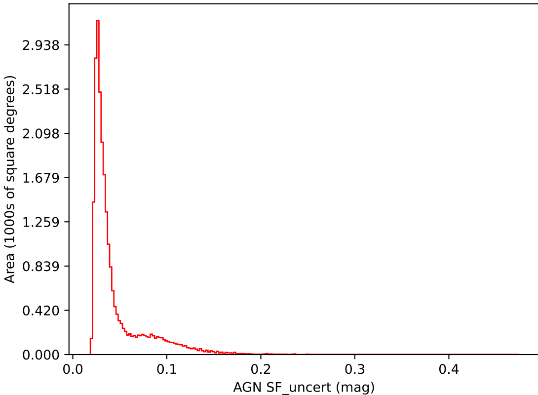
weather_cloudso12v3.4_10yrs i band: AGN SF_uncert
