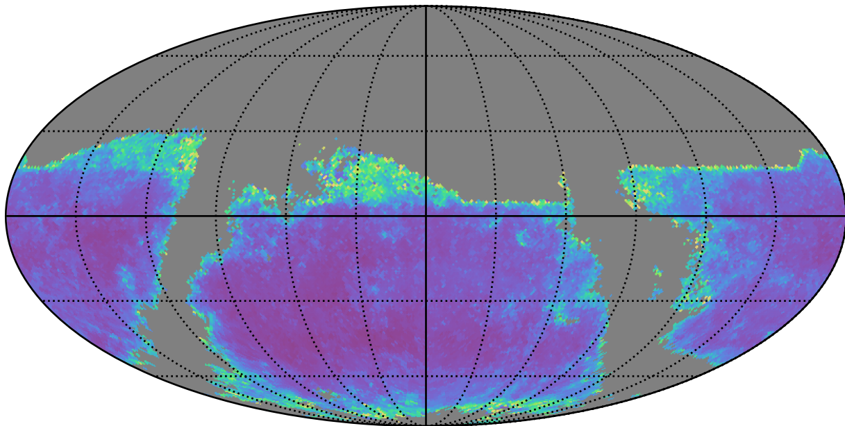
weather_cloudso12v3.4_10yrs g band: AGN SF_uncert
