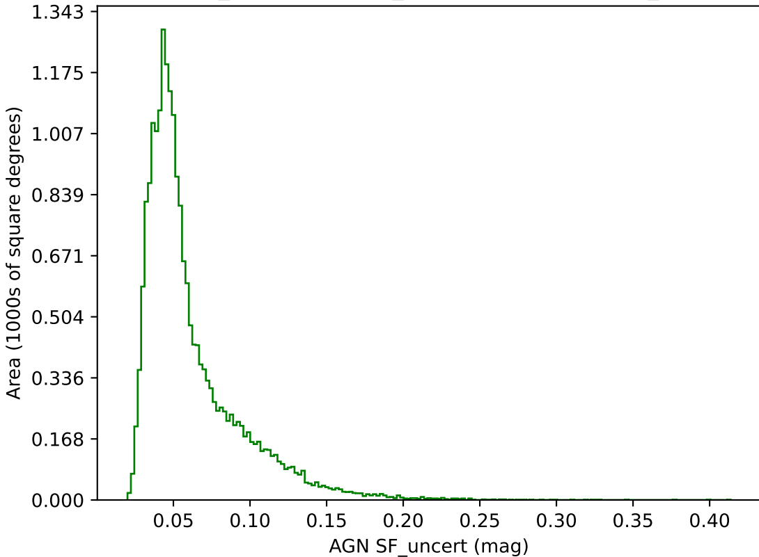
weather_cloudso12v3.4_10yrs g band: AGN SF_uncert
