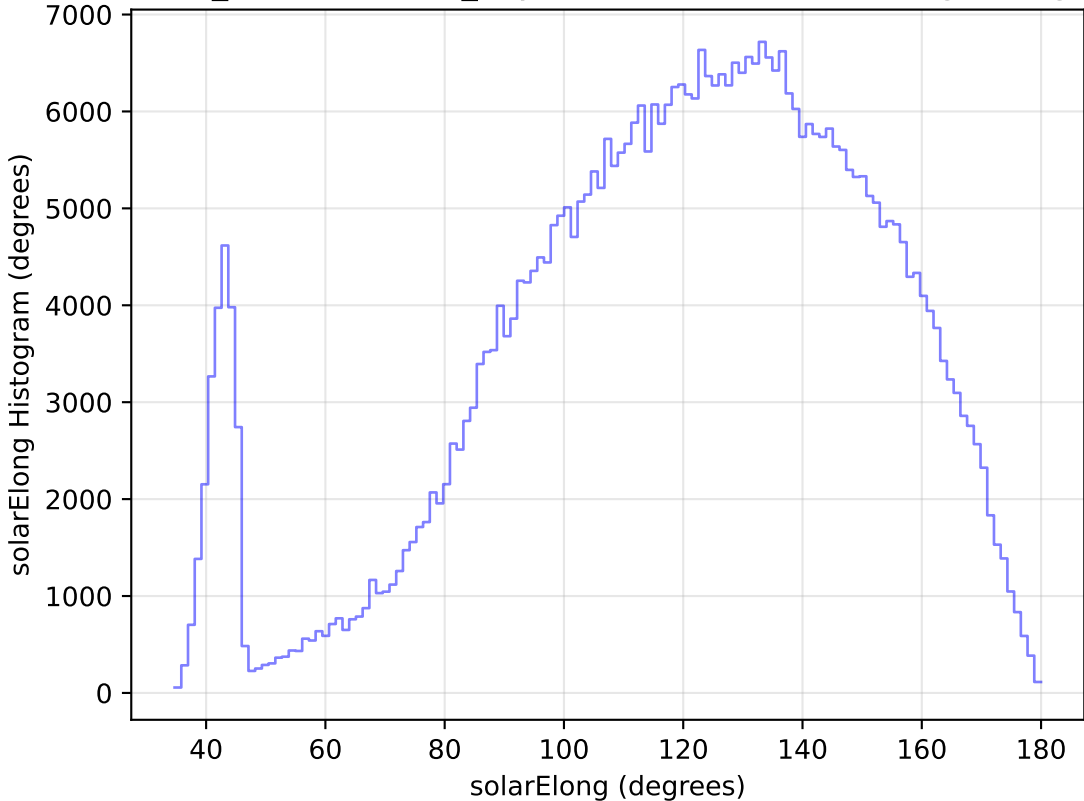
weather_cloudso12v3.4_10yrs WFD z band: solarElong Histogram
