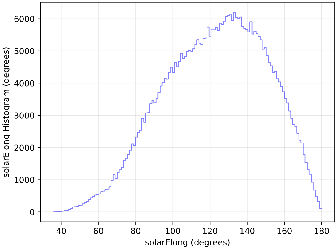
weather_cloudso12v3.4_10yrs WFD y band: solarElong Histogram
