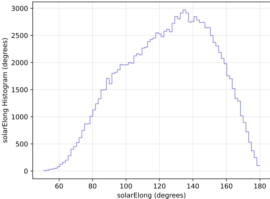
weather_cloudso12v3.4_10yrs WFD u band: solarElong Histogram
