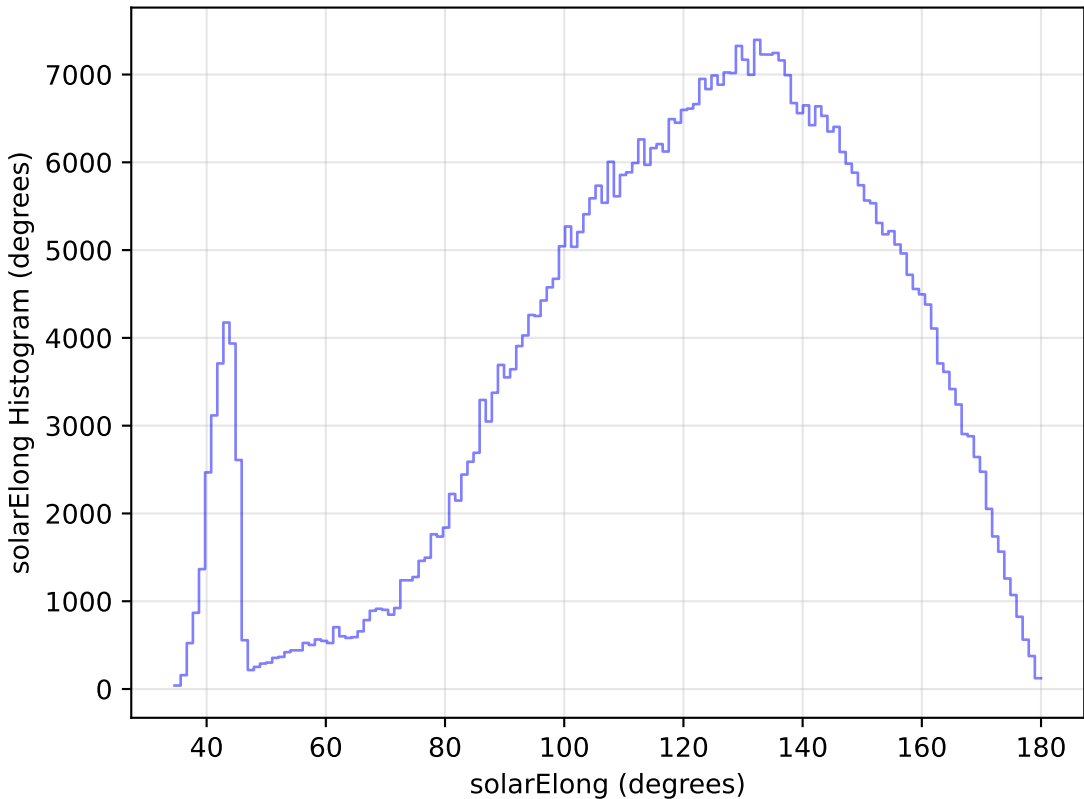
weather_cloudso12v3.4_10yrs WFD i band: solarElong Histogram
