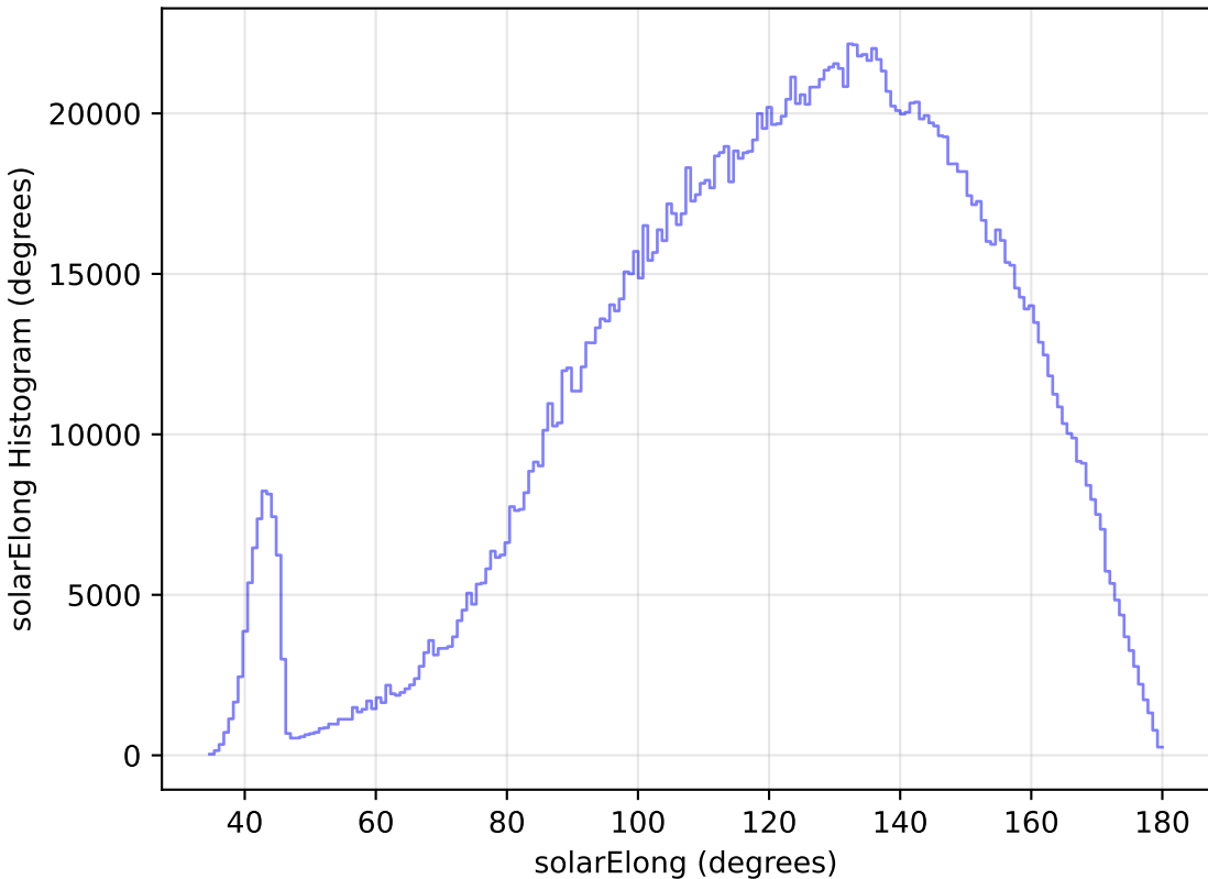
weather_cloudso12v3.4_10yrs WFD all bands: solarElong Histogram
