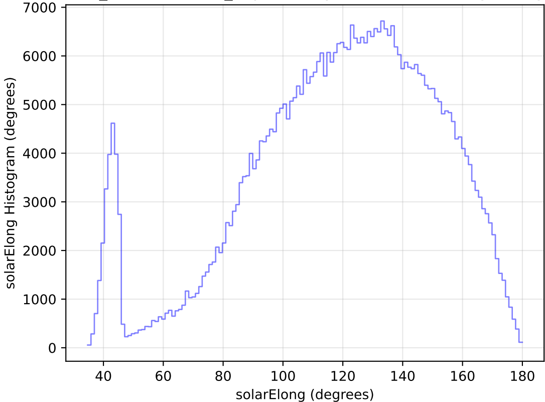
weather_cloudso12v3.4_10yrs All sky z band: solarElong Histogram
