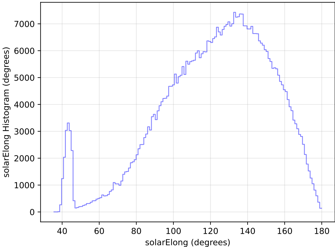
weather_cloudso12v3.4_10yrs All sky r band: solarElong Histogram
