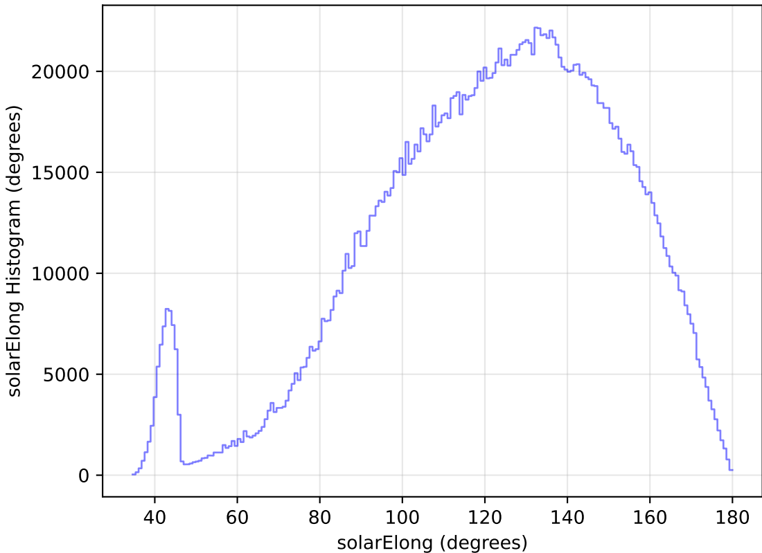
weather_cloudso12v3.4_10yrs All sky all bands: solarElong Histogram
