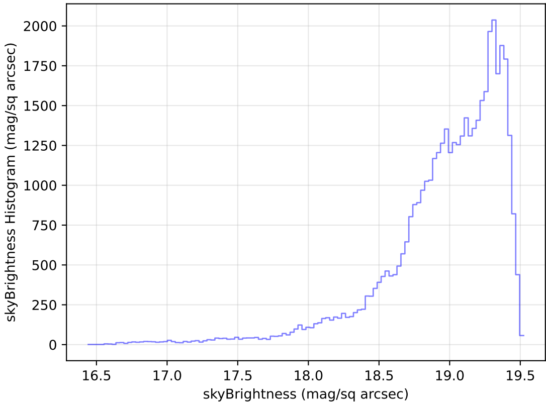
weather_cloudso12v3.4_10yrs Yr 1 z band: skyBrightness Histogram
