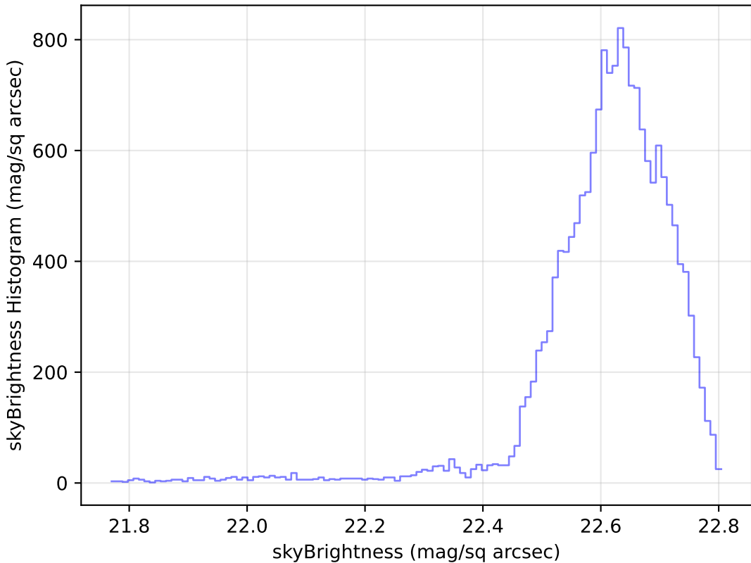
weather_cloudso12v3.4_10yrs Yr 1 u band: skyBrightness Histogram
