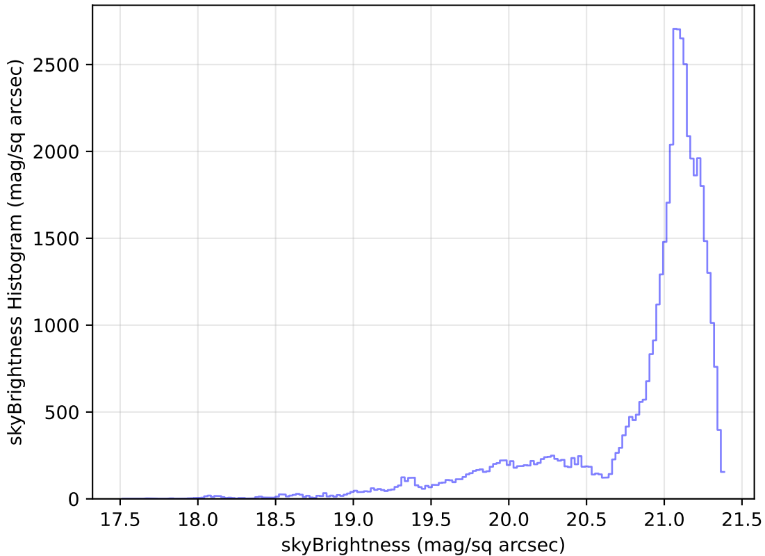
weather_cloudso12v3.4_10yrs Yr 1 r band: skyBrightness Histogram
