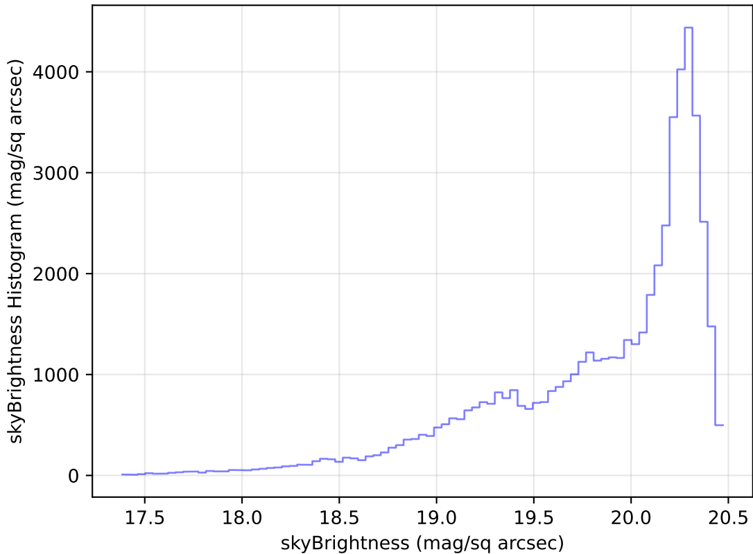
weather_cloudso12v3.4_10yrs Yr 1 i band: skyBrightness Histogram
