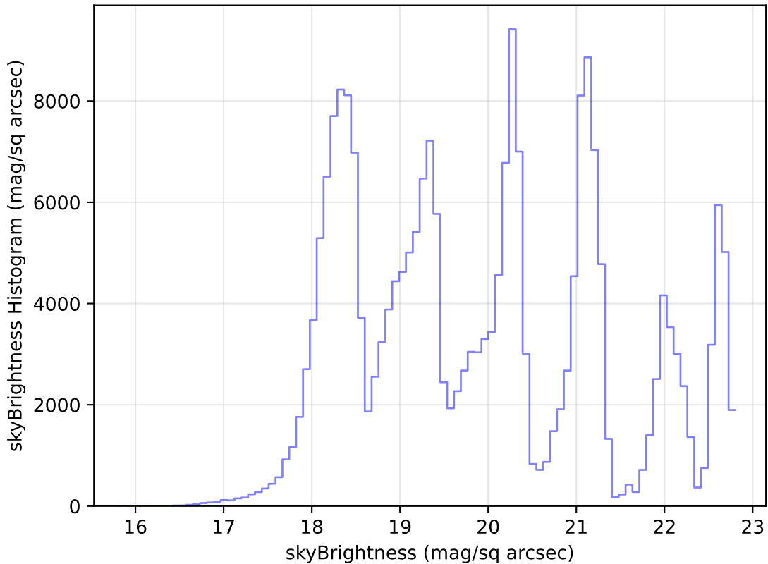
weather_cloudso12v3.4_10yrs Yr 1 all bands: skyBrightness Histogram
