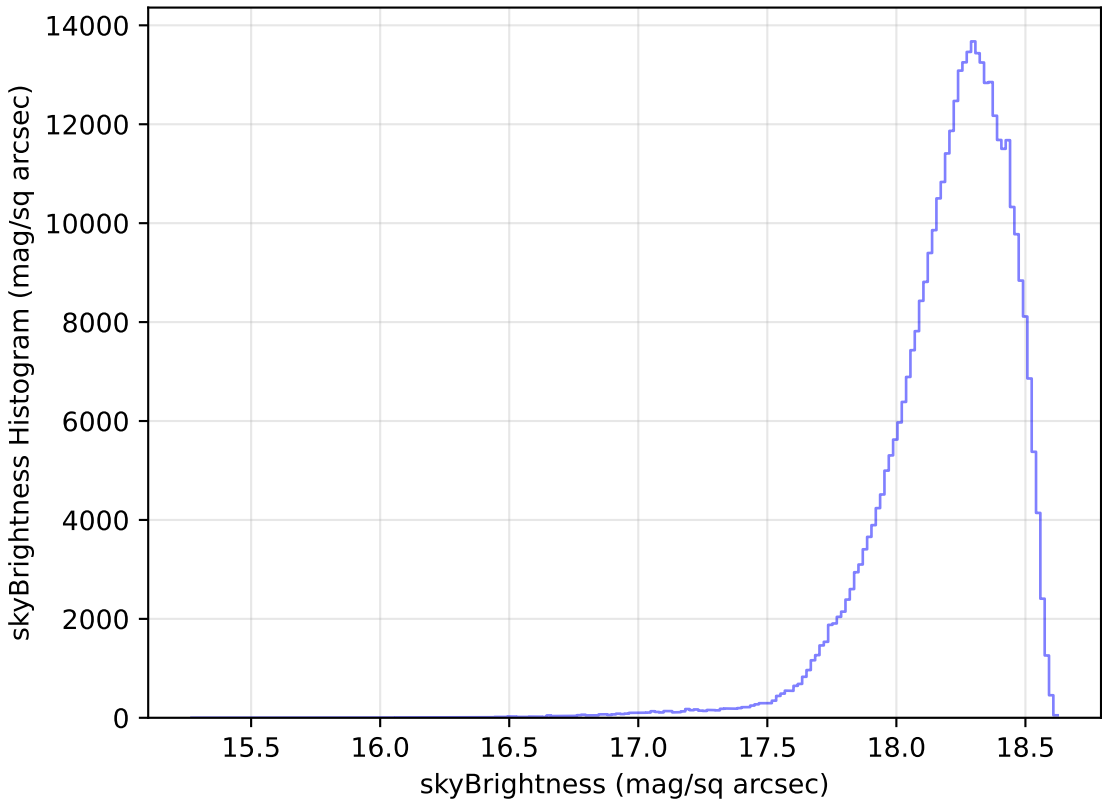
weather_cloudso12v3.4_10yrs WFD y band: skyBrightness Histogram
