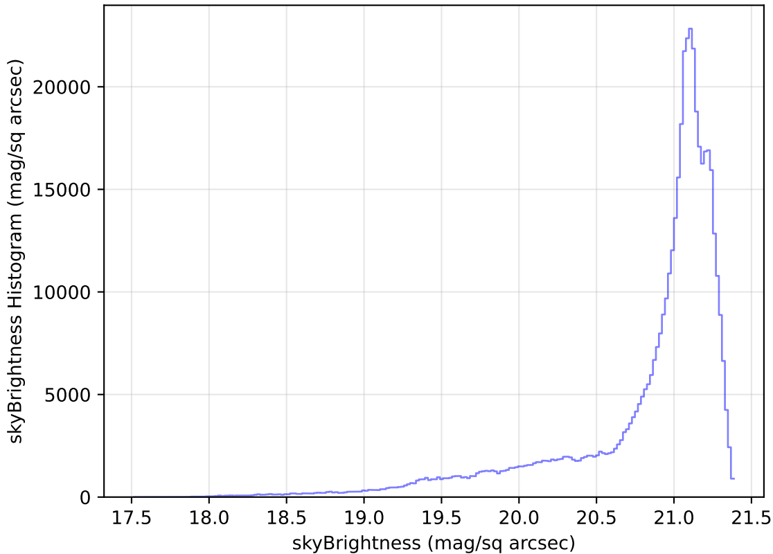
weather_cloudso12v3.4_10yrs WFD r band: skyBrightness Histogram
